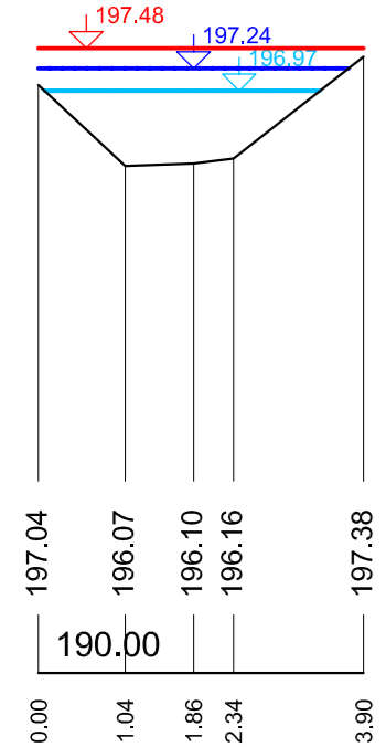
P 2 - 0.01100 km
